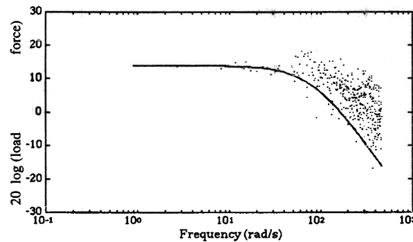
Figure 6: Theoretical and experimental force amplification ratio along the horizontal direction.
