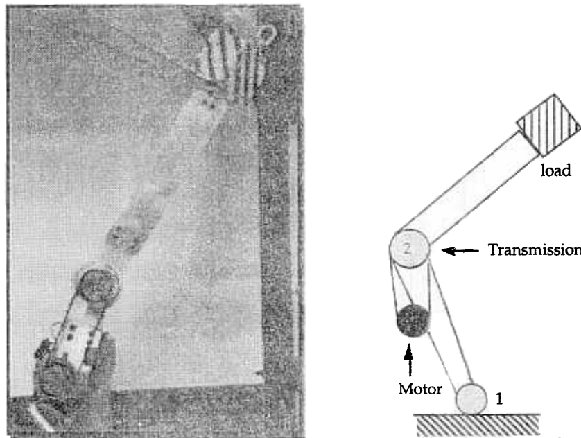
Figure 5: An experimental walking machine consisting of two links. Only one joint is powered. The goal of our research has been to stabilize this under actuated system.
