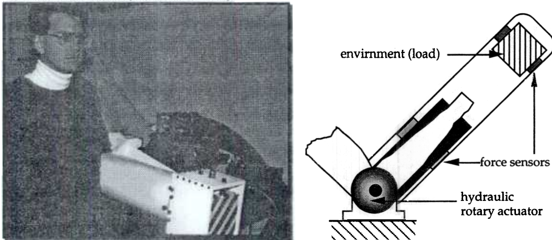
Figure 2: A one-degree-of-freedom hydraulic extender during an unconstrained maneuver.
