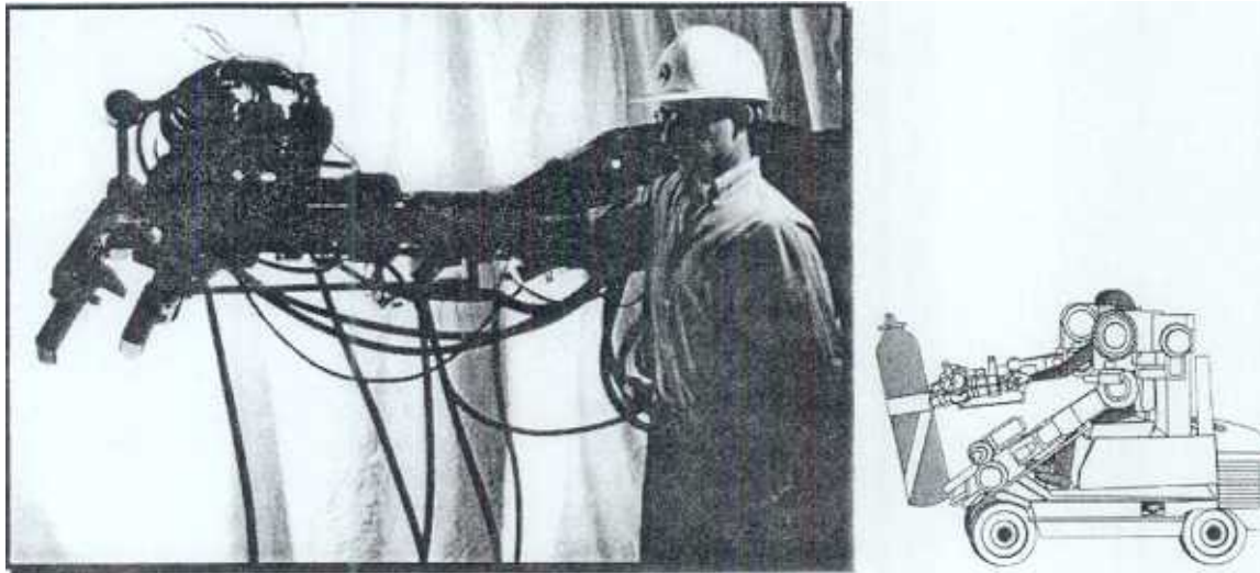
Figure 1: Experimental Six-Degree-of-Freedom Hydraulic Extender designed at UC, Berkeley.
