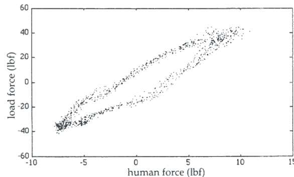
Figure 7: Load force versus human force along the horizontal direction. Slope is approximately 5.
