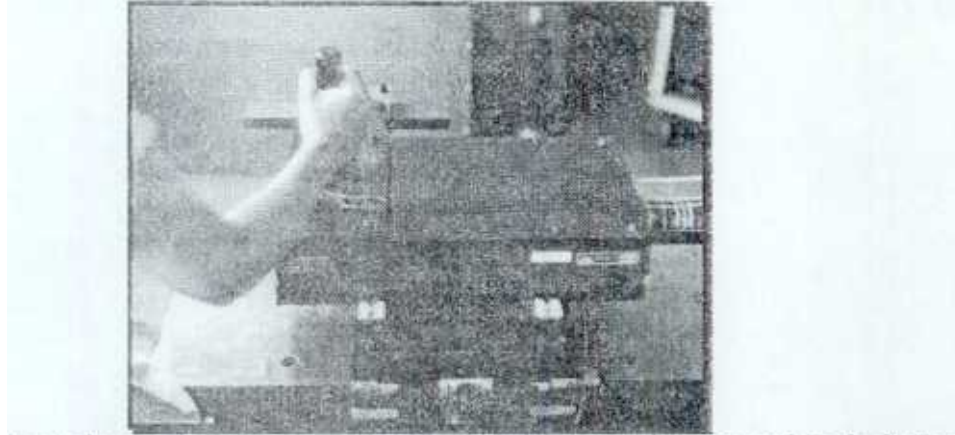
Figure 4: To understand significant variations in human arm dynamics when the human wears an extender, a computer-driven XY table was designed and built for measuring the human arm dynamics in horizontal maneuvers
