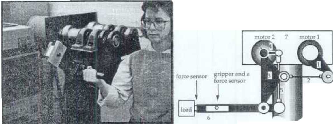
Figure 3: A two-degree-of-freedom direct-drive experimental extender to verify the feasibility of using direct-drive actuators for high-speed maneuvers of loads weighing less than 50 lb.
